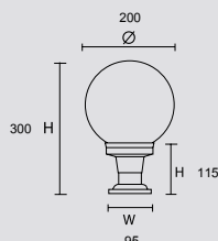
MODEL DRAWING
