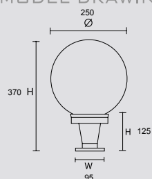
MODEL DRAWING
