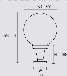
MODEL DRAWING
