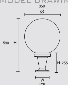
MODEL DRAWING
